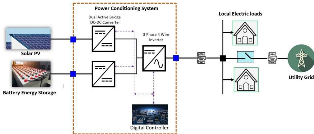
Fig 2. Block diagram of Microgrid PCS
