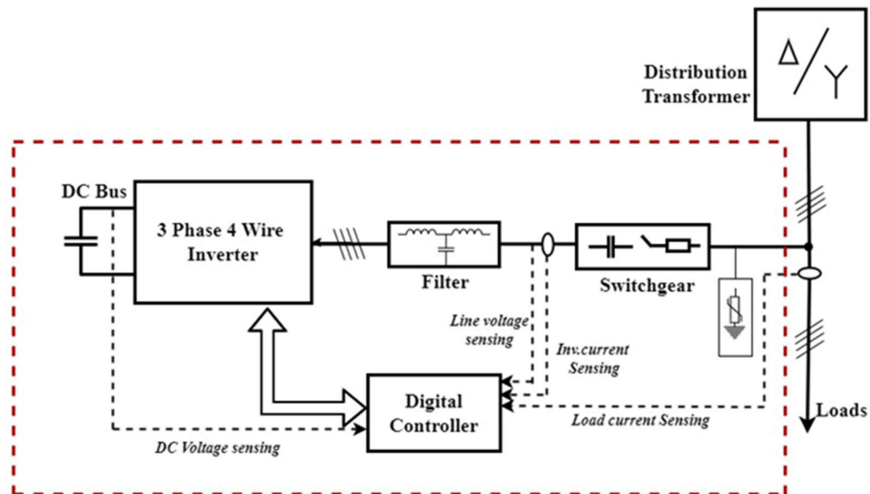
Fig 2. Building blocks of STATCOM
