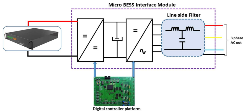
Fig 2. Scheme of Micro BESS Interface module
