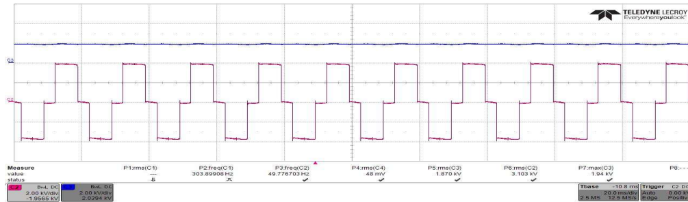
Fig.2. Three-level line to line voltage = 3.1kV at 50 Hz (Square wave mode of operation) Main DC link voltage = 1.94kV
