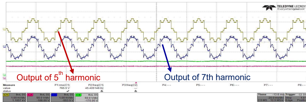
Fig.3. 5th and 7th Harmonic Compensated voltages
