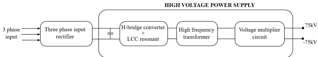
Fig.1 Block diagram of High Voltage Power Supply
