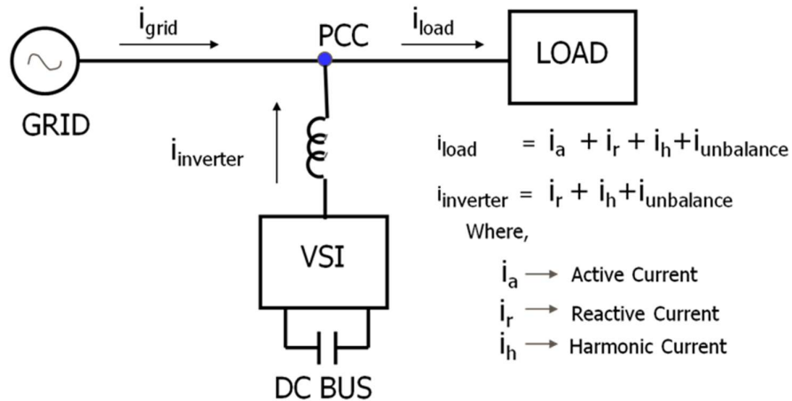
Fig. 1: Shunt connected system for PQ improvement in grid
