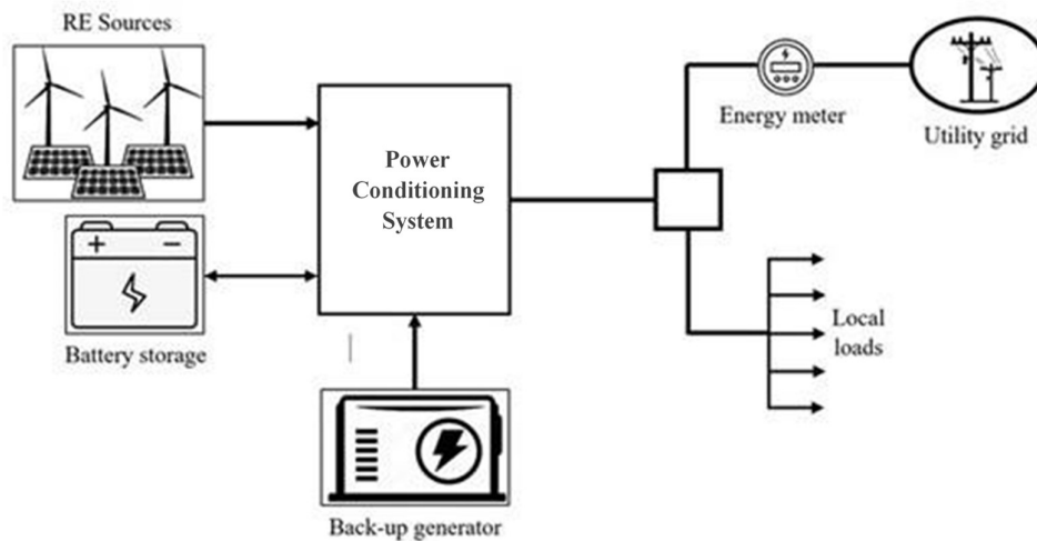
Fig 1. Basic structure of a green microgrid
