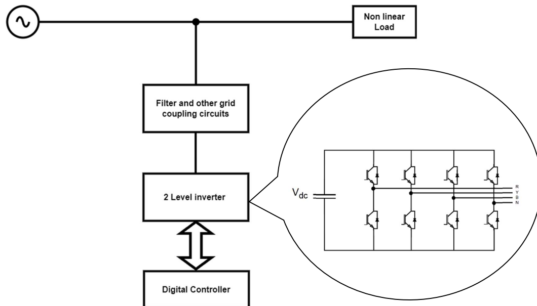
Fig. 3 : Two level Inverter based STATCOM
